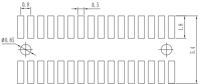
PCB LAYOUT
