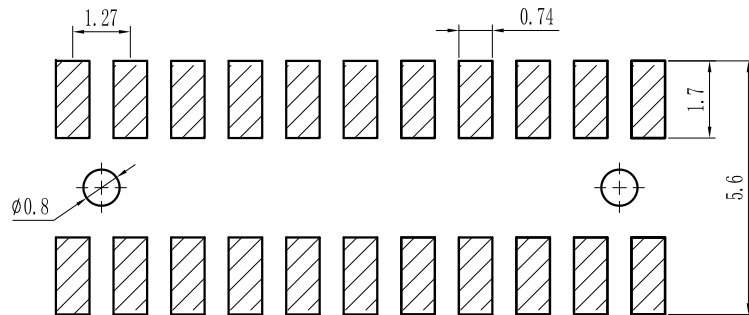
PCB LAYOUT
