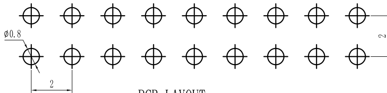
PCB LAYOUT
