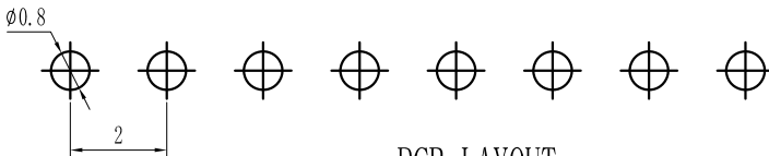
PCB LAYOUT
