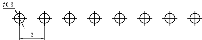
PCB LAYOUT
