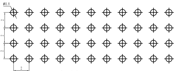
PCB LAYOUT
