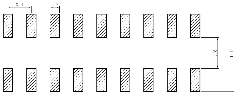
PCB LAYOUT
