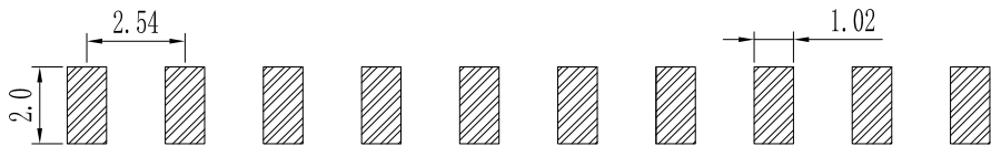
PCB LAYOUT
