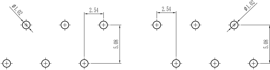
A Type PCB LAYOUT B Type
