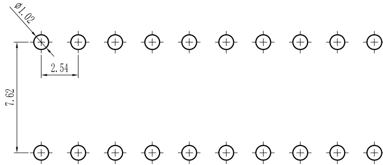
PCB LAYOUT
