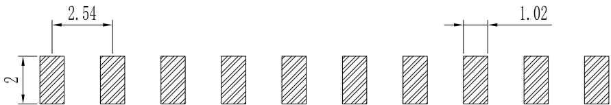
PCB LAYOUT
