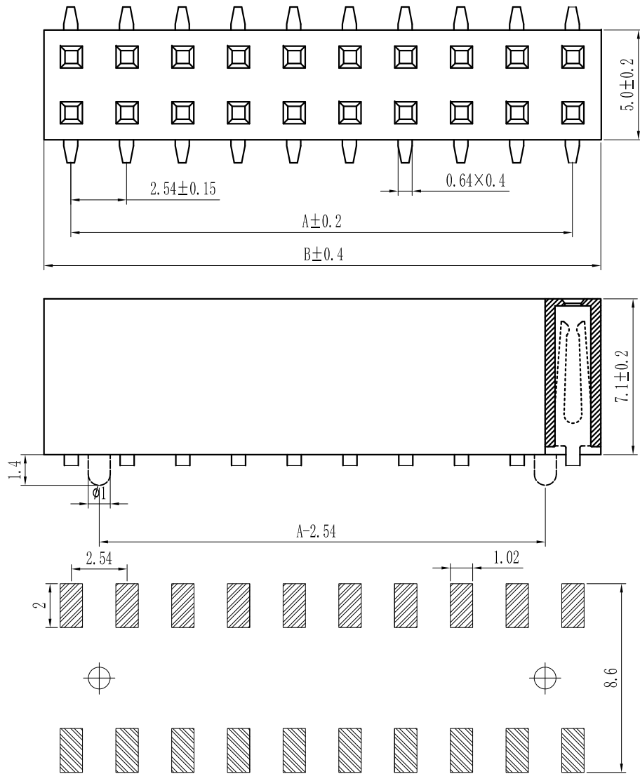
PCB LAYOUT
