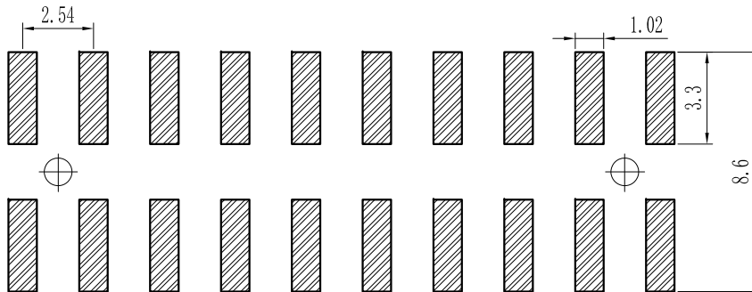
PCB LAYOUT
