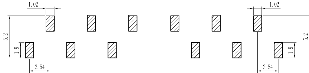
A Type B Type PCB LAYOUT
