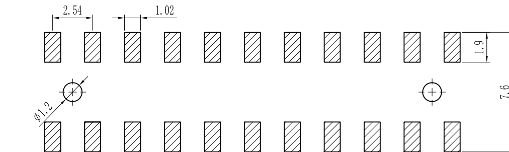
PCB LAYOUT
