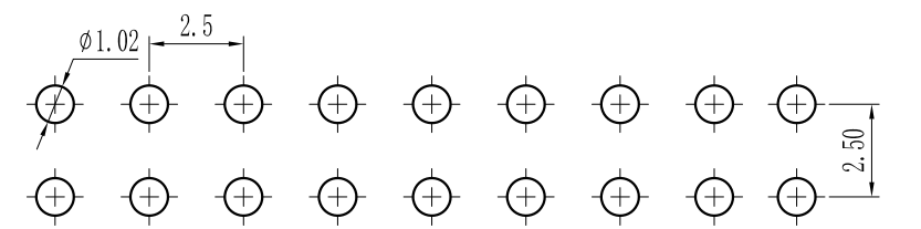
PCB LAYOUT
