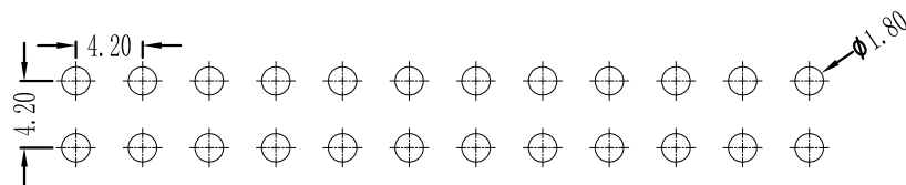
PCB LAYOUT
